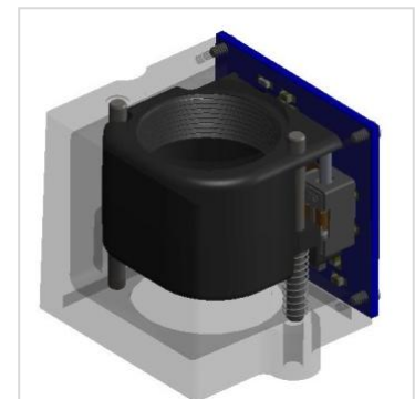
M3-F has pin-bushing guides for lens motion.
